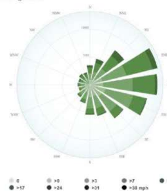
prevailing winds
